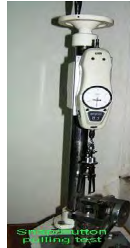
Photo 32 ) Button pulling test
